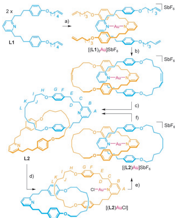
Scheme 2. Gold(I)-template catenane synthesis and subsequent chemistry. a) 1. AuCl(SMe 2 ), acetone, 5 min; 2. AgSbF 6 , 5 min; b) [(PCy 3 ) 2 Cl 2 Ru=CHPh], CH 2 Cl 2 , 2 d; c) 1. 1 M HCl(aq.)/CH 2 Cl 2 (1:1), 40 °C, 18 h; 2. H 2 , Pd/C, THF/EtOH (1:1), 18 h; L2 (41 % from L1 ); d) AuCl(SMe 2 ), acetone, 5 min; e) AgSbF 6 , acetone, 5 min; > 98 %; f) 1 M HCl(aq.)/CH 2 Cl 2 (1:1), 40 °C, 18 h or hν 400–700 nm (500 W halogen lamp), CHCl 3 , 6 d; > 98 %.
