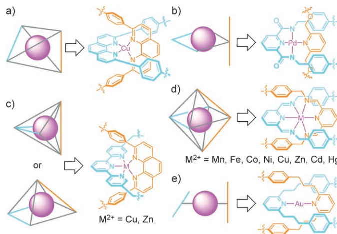
Scheme 1. Metal coordination geometries successfully utilized in the metal-template synthesis of catenanes and rotaxanes. a) Four-coordinate (tetrahedral); [3a,4e,5a,b,6,8c,9a,b,11] b) four-coordinate (square planar); [5d,9c,13] c) five-coordinate (square-based pyramidal/trigonal bipyramidal); [14] d) six-coordinate (octahedral); [8a,b,12] e) two-coordinate (linear; this work).
