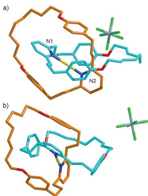
Figure 3. X-ray crystal structure [22] of gold(I) catenate [(\mathbf{L2})\text{Au}]\text{SbF}_6 , viewed a) parallel to the N–Au–N bond, b) close to the axis of the N–Au–N bond. Carbon atoms are shown in light blue for one macrocycle and in brown for the other; O red, N blue, Au I gold, Sb grey, F green. Selected bond lengths [Å] and angles [°]: N1–Au 2.05, N2–Au 2.06; N1–Au–N2 175.3; closest Au...Au contact 11.31 Å.
