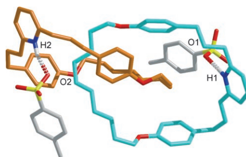
Figure 2. Molecular structure [21] of H 2 L2 (OTs) 2 from X-ray structure analysis of a single crystal grown by vapor diffusion of diisopropyl ether into a saturated acetone solution. Carbon atoms are shown in light blue for one macrocycle and in brown for the other; O red, N blue, S yellow. Hydrogen bond lengths [Å] and angles [°]: NH1...O1 = NH2...O2 1.76; N1-H1-O1 = N2-H2-O2 163.
