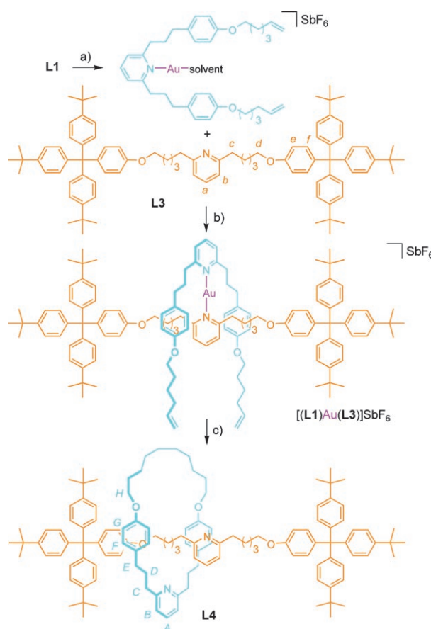
Scheme 3. Gold(I)-template rotaxane synthesis. a) 1. \text{AuCl}(\text{SMe}_2) , acetone, 5 min; 2. \text{AgSbF}_6 , acetone, 5 min; b) acetone, 5 min; c) 1. [(\text{PCy}_3)_2\text{Cl}_2\text{Ru}=\text{CHPh}] , \text{CH}_2\text{Cl}_2 , 2 d; 2. 1 M \text{HCl}(\text{aq})/\text{CH}_2\text{Cl}_2 (1:1), 40^\circ\text{C} , 18 h; 3. \text{H}_2 , \text{Pd/C} , \text{THF}/\text{EtOH} (1:1), 18 h, L4 (26% from L1 ).
