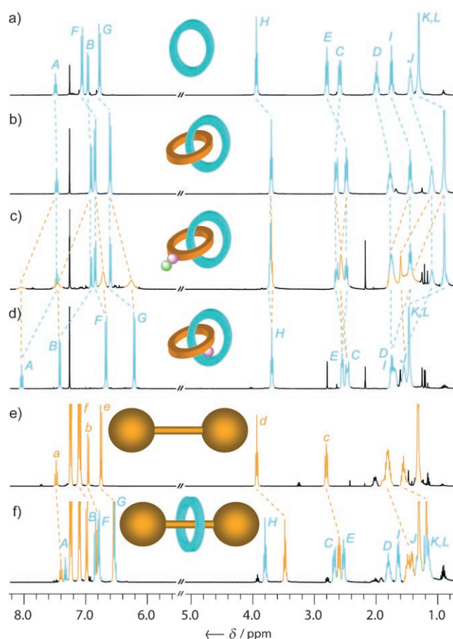
Figure 1. 1 H NMR spectra (400 MHz, CDCl 3 , 300 K) of a) the non-interlocked macrocycle; b) the metal-free catenane L2 ; c) [( L2 )Au]Cl; d) gold(I) catenane [( L2 )Au]SbF 6 ; e) thread L3 , and f) the metal-free rotaxane L4 . The assignments correspond to the lettering shown in Schemes 2 and 3.
